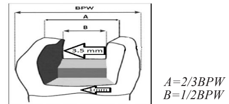
Fig.2. dimensions of the prepared MOD cavity
