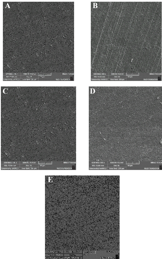
Figure 1. SEM images of composite resin after treatment ( \times 500 ): (A) White Now, (B) Optic White, (C) Opalescence, (D) Max Fresh and (E) control.
