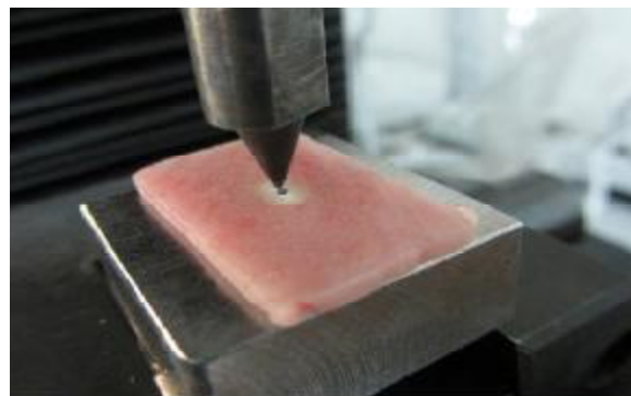
Figure.1: push-out bond strength test
