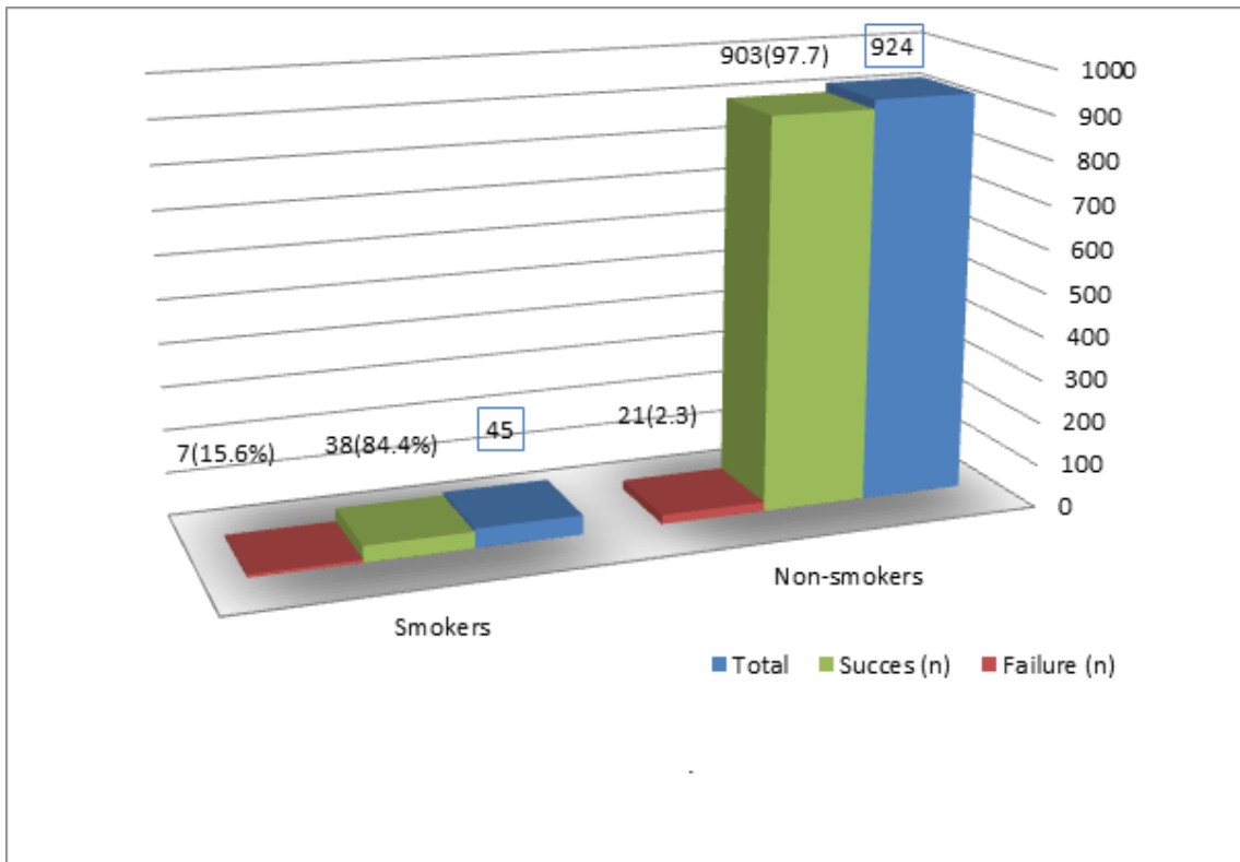
Figure 2. prevalence of implant failure rate in smokers and nonsmokers. significant failure rate was found among smokers. (Fisher Exact test, p < 0.05 )
